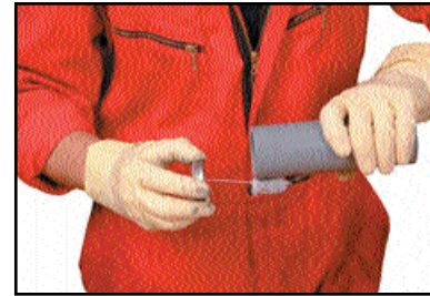
Applying the primer to the pipe
